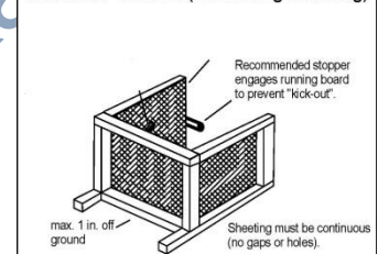
WARM-UP STAND (not a design drawing)
